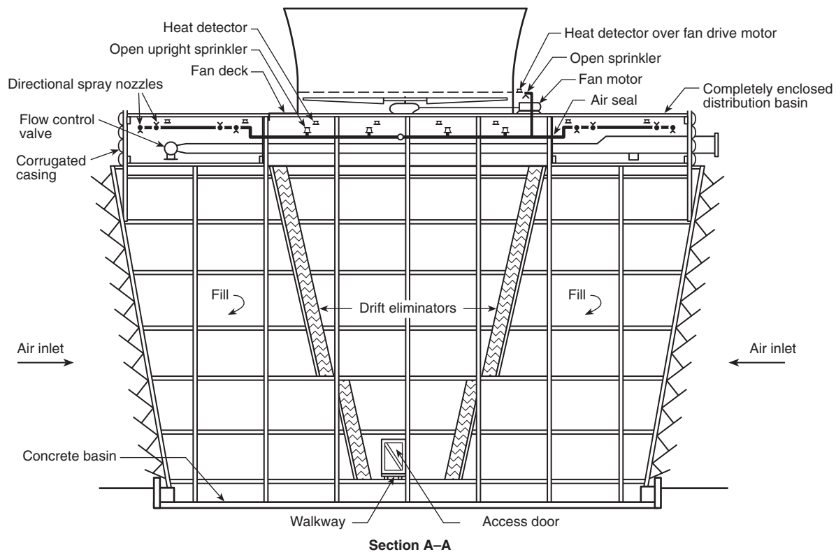
FIGURE A.21.24.2.3(b) Section View, Typical Deluge Fire Protection Arrangement for Crossflow Towers with Completely Enclosed Distribution Basins. [214:Figure A.5.2.4.3(b)]
