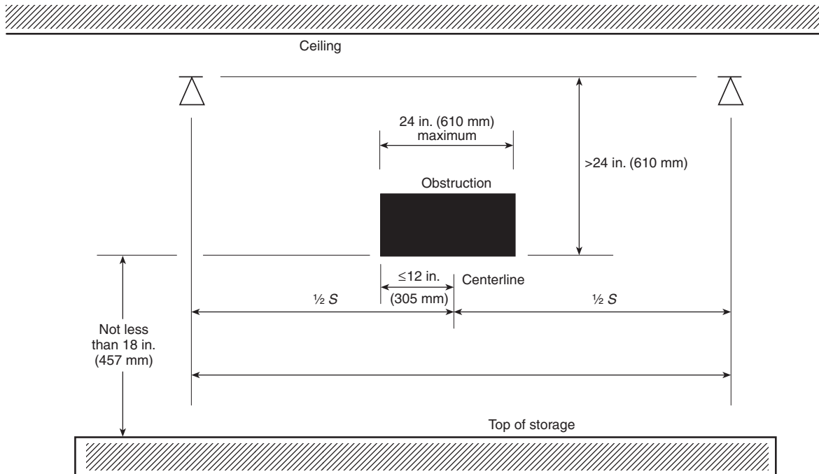
FIGURE 8.11.5.3.4 Obstruction More Than 24 in. (610 mm) Below the Sprinkler (Large Drop Sprinkler).
