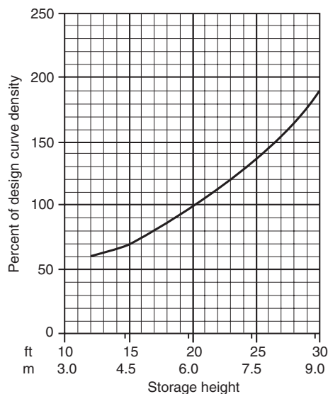
FIGURE 14.2.4.3 Ceiling Sprinkler Density vs. Storage Height.
