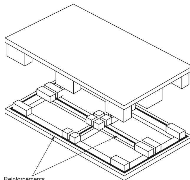
FIGURE A.3.9.1.17(a) Cut-Away Reinforced Plastic Pallet.
