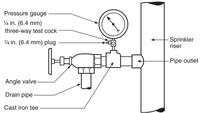
FIGURE A.8.16.2.4 Unacceptable Pressure Gauge Location.
