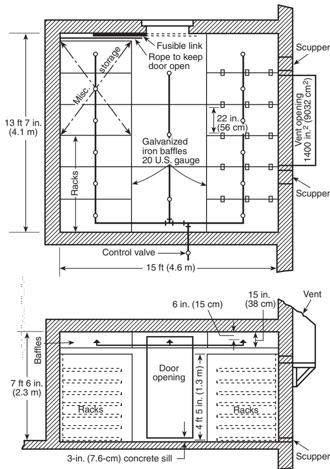
FIGURE 21.8.2(a) Raw Stock Storage Vault Showing General Arrangement of Sprinklers, Racks, and Baffles. [42:Figure 6.3.3.7(a)]
