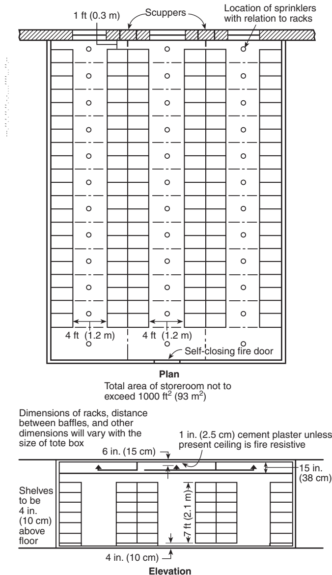
FIGURE 21.8.2.5(a) Tote Box Storeroom Showing General Arrangement of Racks and Sprinklers. [42:Figure 6.7]
