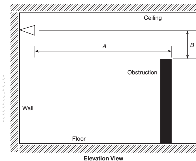
FIGURE 8.9.5.2.2 Suspended or Floor-Mounted Obstructions (Extended Coverage Sidewall Sprinklers) in Light Hazard Occupancies Only.
