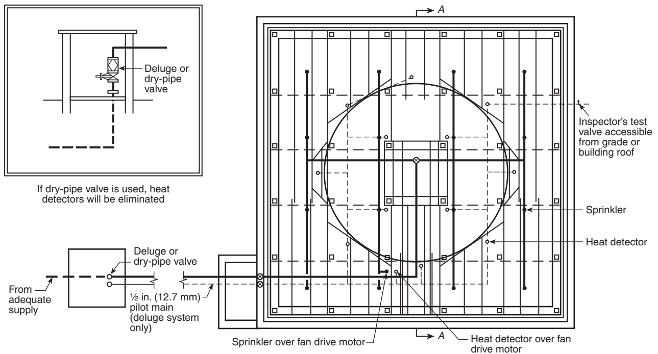
FIGURE A.21.24.2.1(c) Plan View, Typical Deluge or Dry Pipe Fire Protection Arrangement for Counterflow Towers. [214:Figure A.5.2.4.1(c)]
