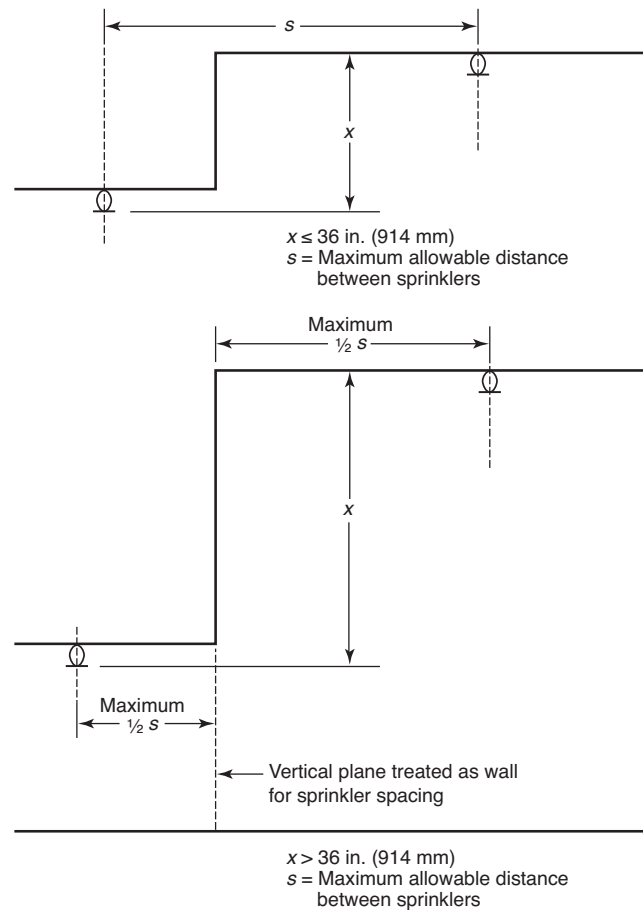
FIGURE 8.6.4.1.1.3 Vertical Changes in Ceiling Elevations.
