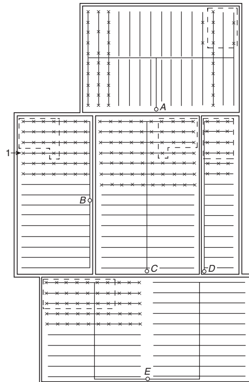
FIGURE A.22.4.4.1(a) Example of Hydraulically Most Demanding Area.
