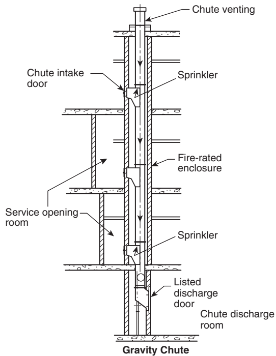
FIGURE A.21.16.2.1(a) Gravity Linen Chute. [82:Figure A.5.2(a)]
