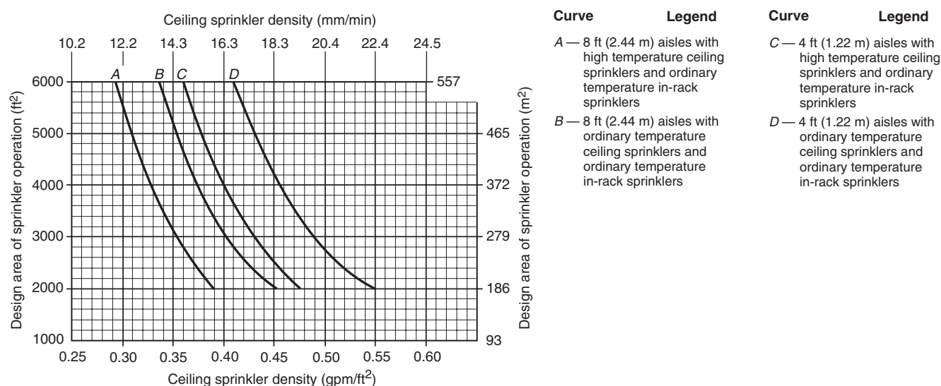
FIGURE 16.2.1.3.2(g) Single- or Double-Row Racks — 20 ft (6.1 m) High Rack Storage — Sprinkler System Design Curves — Class IV Encapsulated Commodities — Conventional Pallets.
