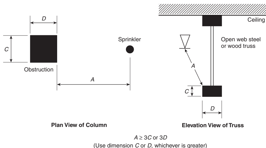
FIGURE 8.11.5.2.1.3 Minimum Distance from Obstruction (Large Drop Sprinkler).
