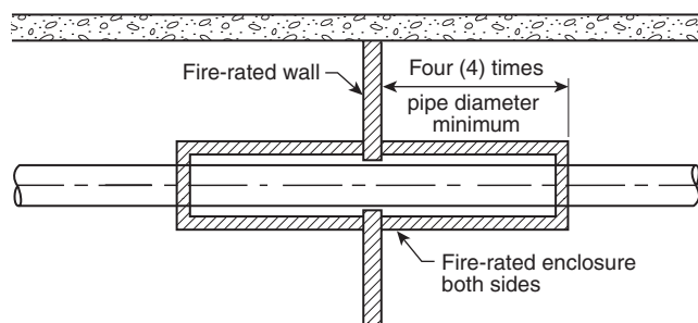
FIGURE A.21.16.2.1(g) Fire Damper Engineering Alternative for Penetration of Wall at Base of Shaft. [82:Figure A.5.3(e)]
