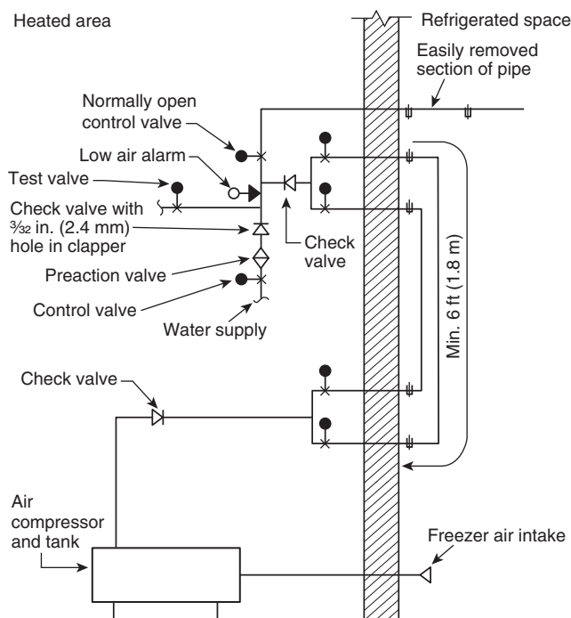
FIGURE 7.9.2.8.4 Valve Arrangement.
