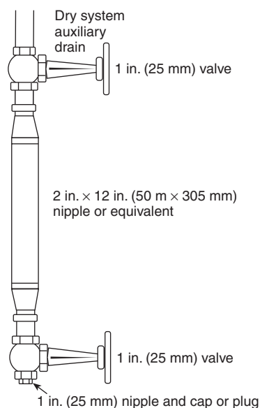
FIGURE 8.16.2.5.3.4 Dry System Auxiliary Drain.
