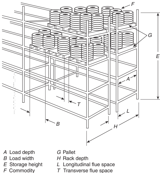
FIGURE A.3.9.4.9(d) Double-Row Fixed Tire Rack Storage.
