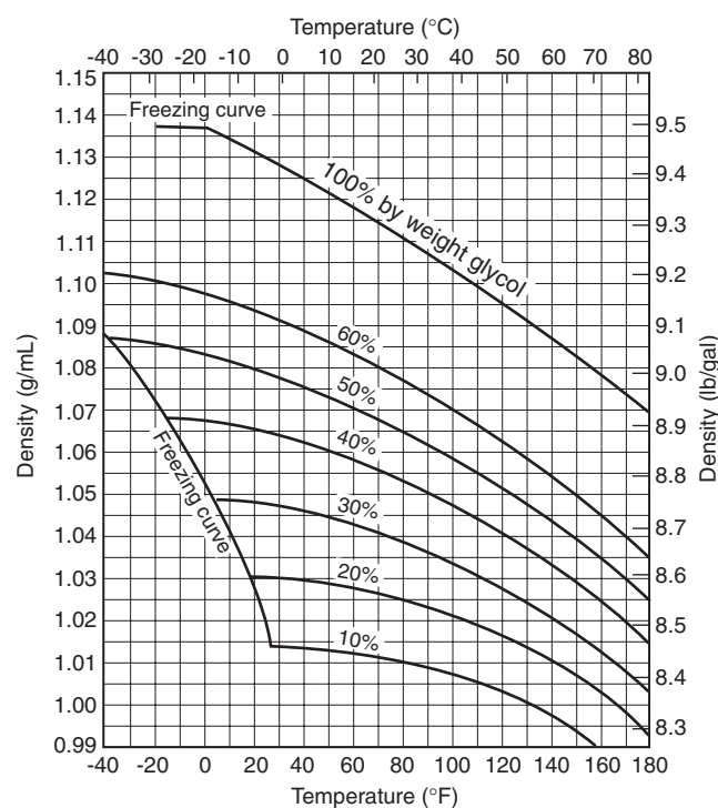
FIGURE 7.6.2.5(b) Densities of Aqueous Propylene Glycol Solutions (Percent by Weight).
