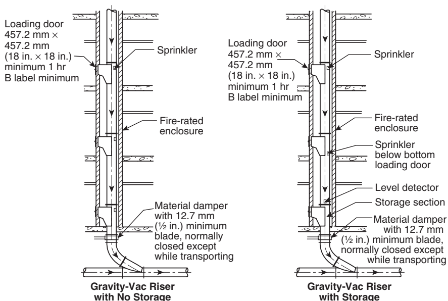
FIGURE A.21.16.2.1(h) Gravity Pneumatic System. [82:Figure A.5.4]
