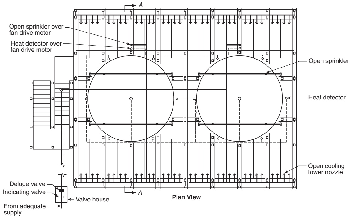
FIGURE A.21.24.2(c) Plan View, Typical Deluge Fire Protection Arrangement for Multicell Crossflow Towers. [214:Figure A.5.2.4.2(c)]
