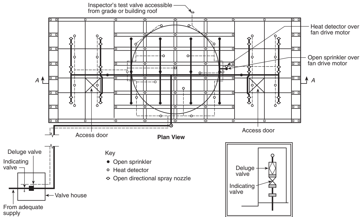
FIGURE A.21.24.2.3(a) Plan View, Typical Deluge Fire Protection Arrangement for Crossflow Towers with Completely Enclosed Distribution Basins. [214:Figure A.5.2.4.3(a)]
