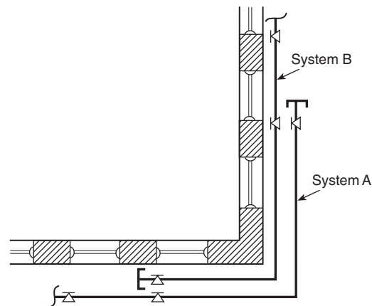
FIGURE 7.8.4.2.1(b) Alternate Arrangement of Check Valves.
