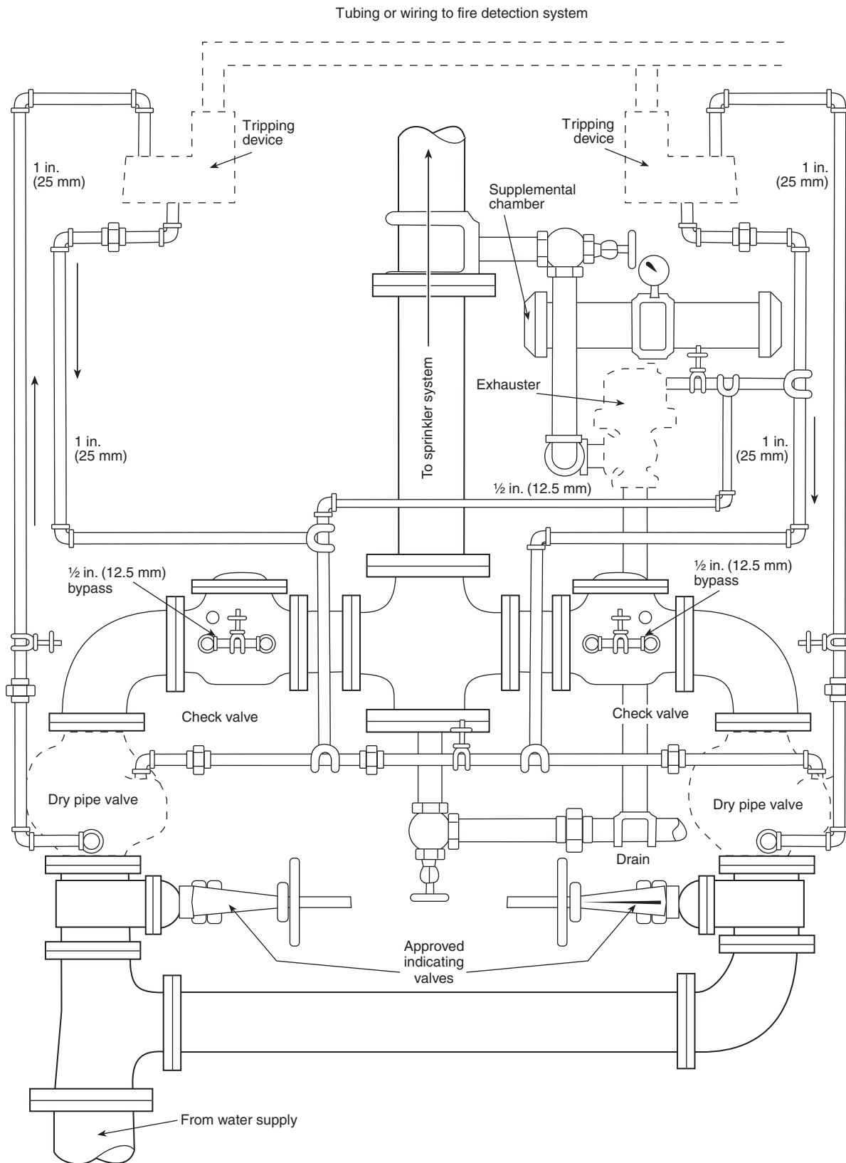
FIGURE 7.4.3.2 Header for Dry Pipe Valves Installed in Parallel for Combined Systems; Standard Trimmings Not Shown. Arrows Indicate Direction of Fluid Flow.
