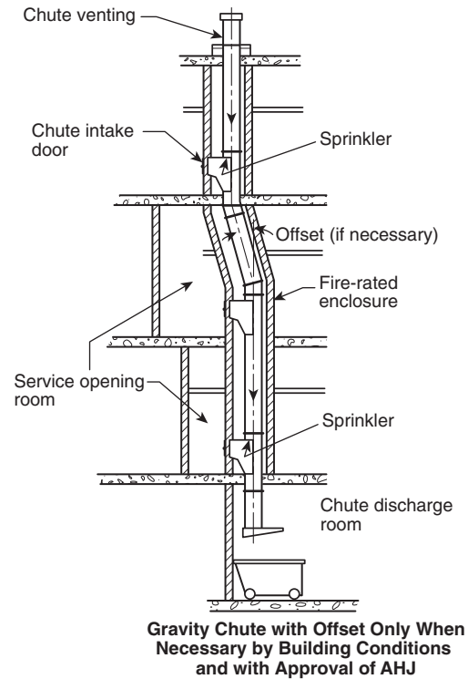
FIGURE A.21.16.2.1(b) Gravity Waste Chute. [82:Figure A.5.2(b)]
