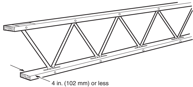
FIGURE A.3.7.2(a) Wood Bar Joist Construction.
