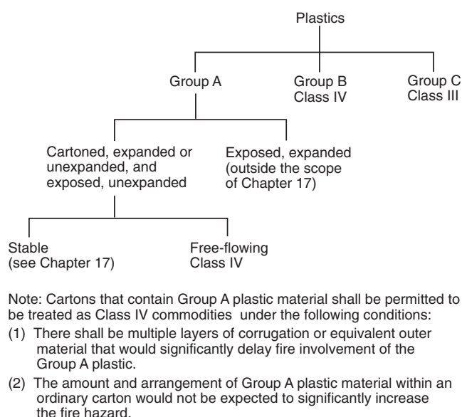
FIGURE 17.1.2.1 Decision Tree.
