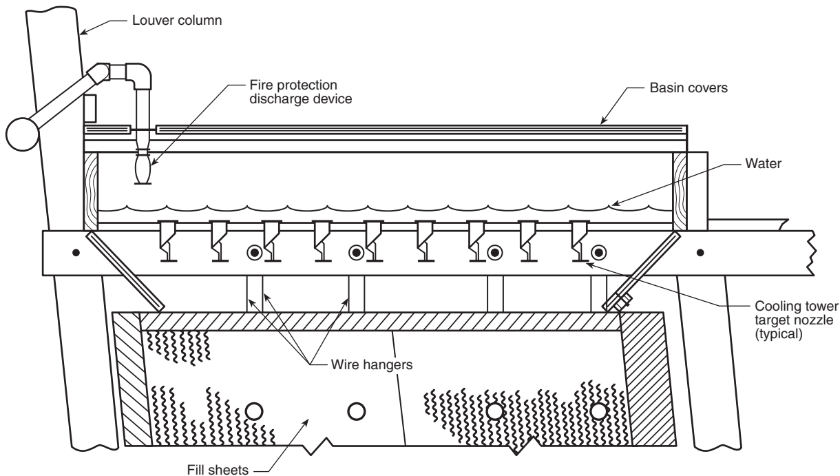
FIGURE A.21.24.2.5 Typical Deluge Fire Protection Arrangement for Crossflow Towers with Covers Completely Enclosing Distribution Basins. [214:Figure A.5.2.4.5]
