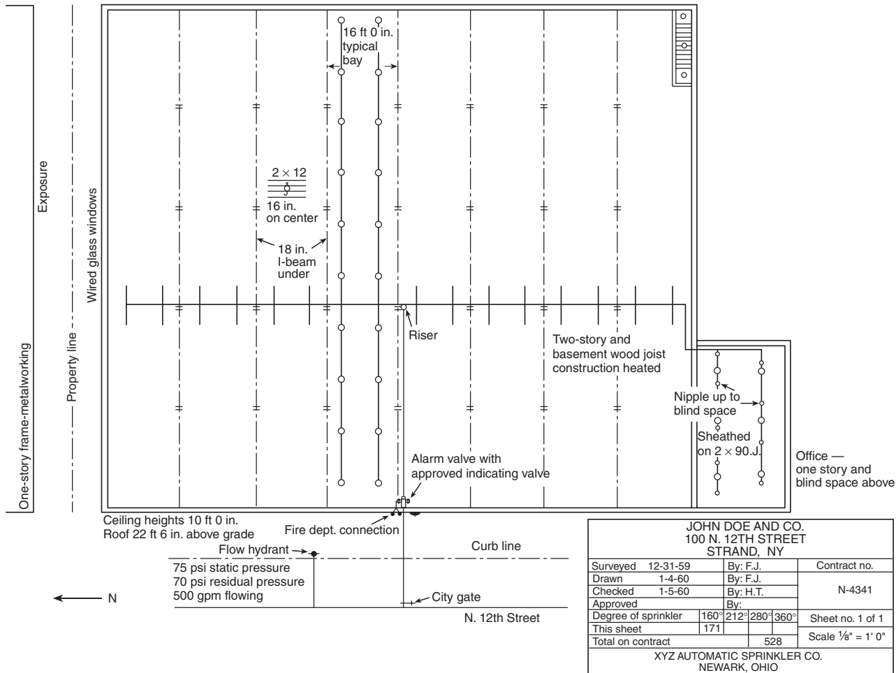
FIGURE A.22.1(a) Typical Preliminary Plan.
