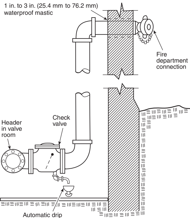
FIGURE 8.17.2.1 Fire Department Connections.
