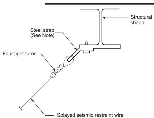
Detail A — At steel beams
