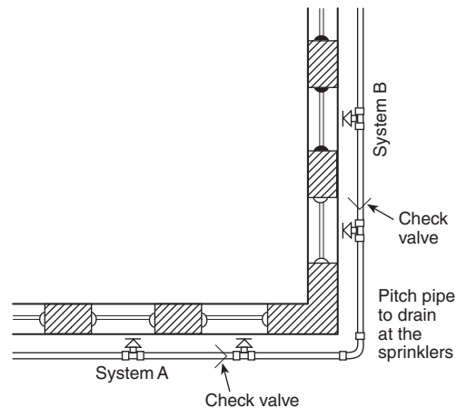
FIGURE 7.8.4.2.1(a) Typical Arrangement of Check Valves.
