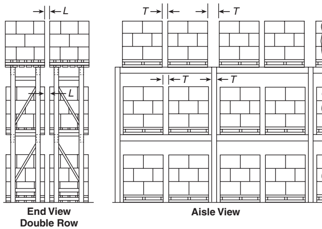
FIGURE A.3.9.3.7(a) Conventional Pallet Rack.
