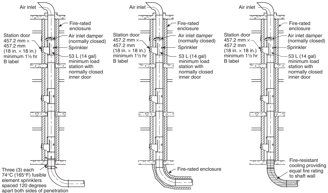
FIGURE A.21.16.2.1(d) Fire Damper Engineering Alternative for Penetration of Floor at Base of Shaft. [82:Figure A.5.3(b)]
