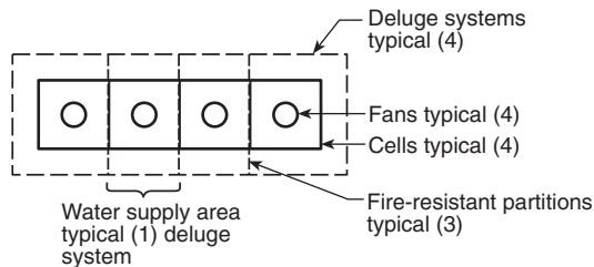
FIGURE A.21.24.1.7.1.3 Multiple Deluge Systems. [214:Figure A.5.6.1.3]
