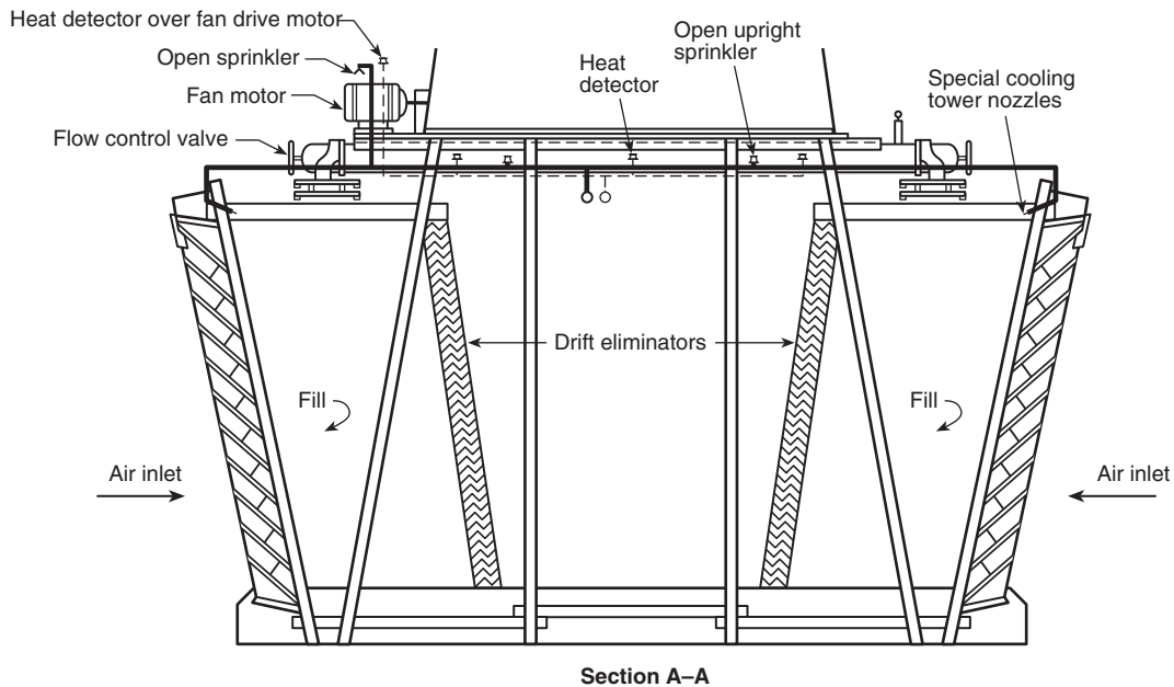
FIGURE A.21.24.2(d) Section View, Typical Deluge Fire Protection Arrangement for Multicell Crossflow Towers. [214:Figure A.5.2.4.2(d)]
