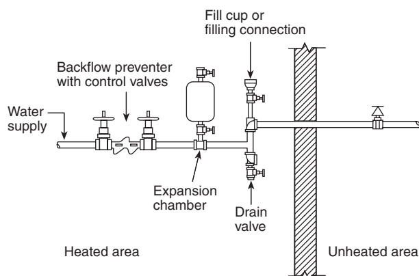
FIGURE 7.6.3.2 Arrangement of Supply Piping with Backflow Device.
