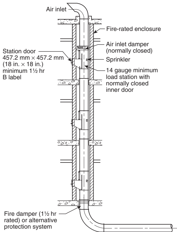
FIGURE A.21.16.2.1(c) Full Pneumatic System. [82:Figure A.5.3(a)]
