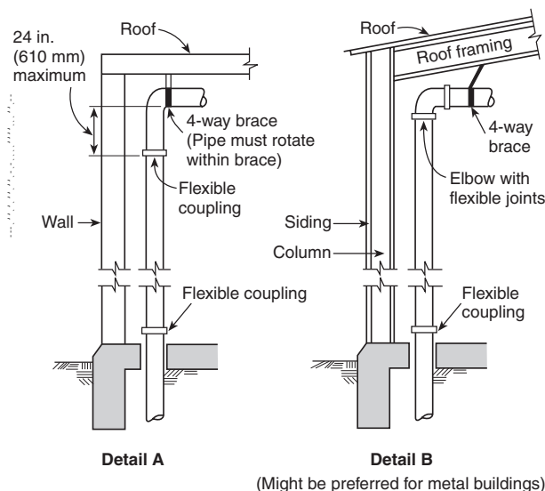
FIGURE A.9.2.3.5.2 Maximum Length of Unsupported Armover Where the Maximum Pressure Exceeds 100 psi (6.9 bar) and a Branch Line Above a Ceiling Supplies Pendent Sprinklers Below the Ceiling.
