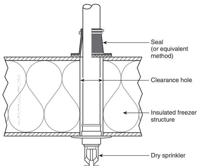
FIGURE A.8.4.10.2(a) Dry Sprinkler Seal Arrangement — Seal on Exterior of Freezer Structure.
