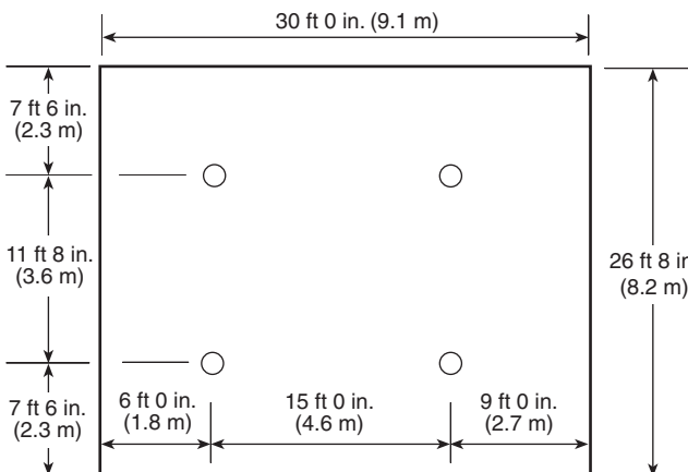
FIGURE A.8.6.3.2.4(d) Small Room Provision — Four Sprinklers.
