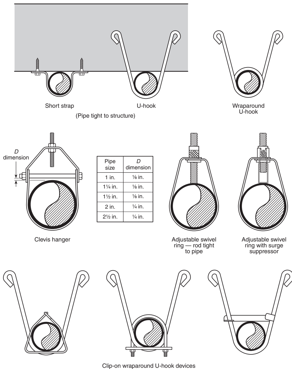
FIGURE A.9.2.3.4(b) Examples of Acceptable Hangers for End-of-Line (or Armoval) Pendant Sprinklers.
