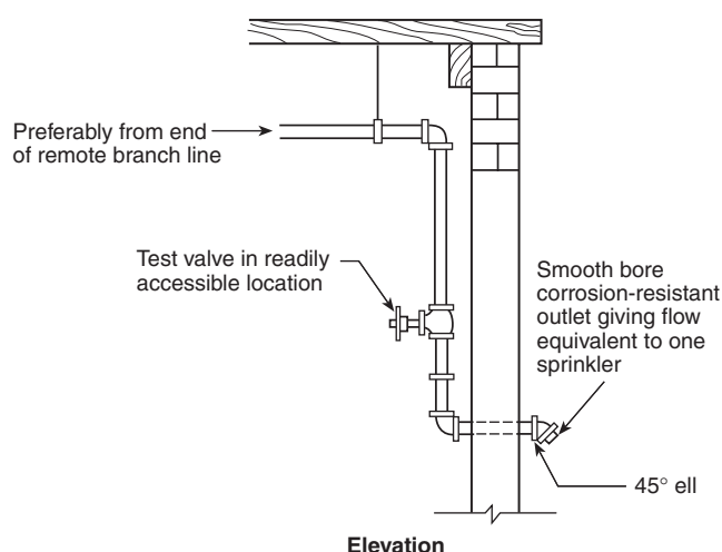
FIGURE A.8.17.4.1 Water Supply Connection with Test Connection.
