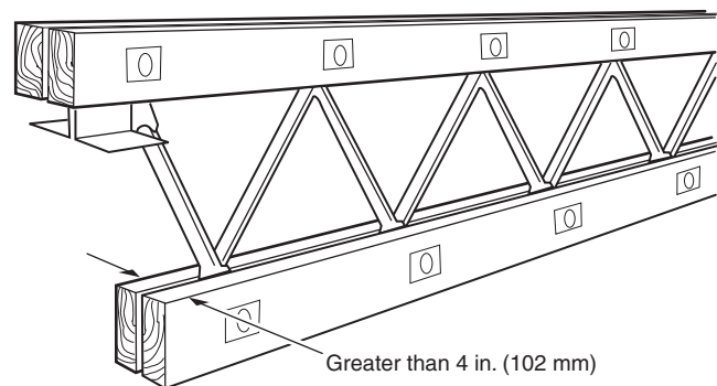
FIGURE A.3.7.2(b) Open-Web Bar Joist Construction.
