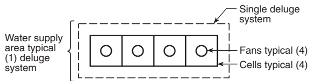
FIGURE A.21.24.1.7.1.1 Single Deluge System. [214:Figure A.5.6.1.1]
