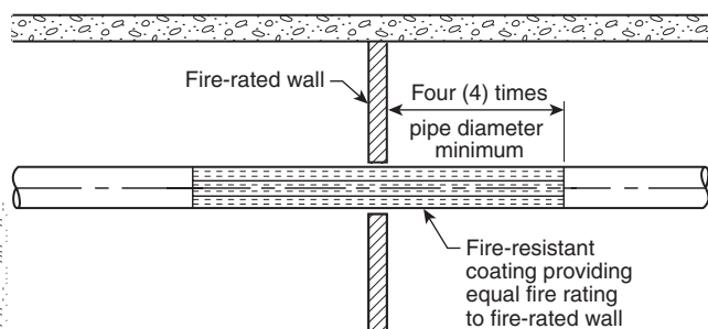
FIGURE A.21.16.2.1(f) Fire Damper Engineering Alternative for Penetration of Fire-Rated Wall. [82:Figure A.5.3(d)]
