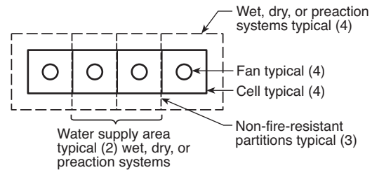
FIGURE A.21.24.1.7.2.2 Multiple Wet, Dry, or Preaction Systems with No Fire-Resistant Partitions. [214:Figure A.5.6.2.2]
