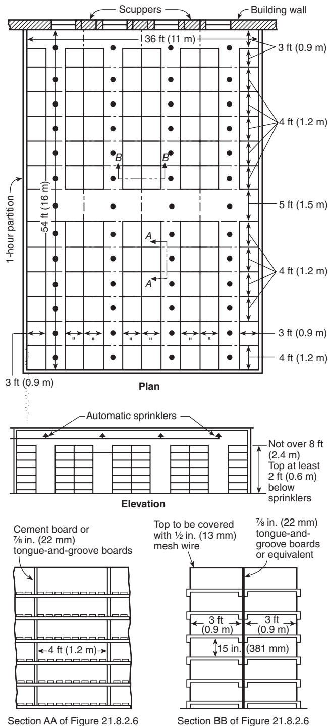
FIGURE 21.8.2.6 Finished-Stock Storeroom Showing General Arrangement of Racks. [42:Figure 6.8(a)]
