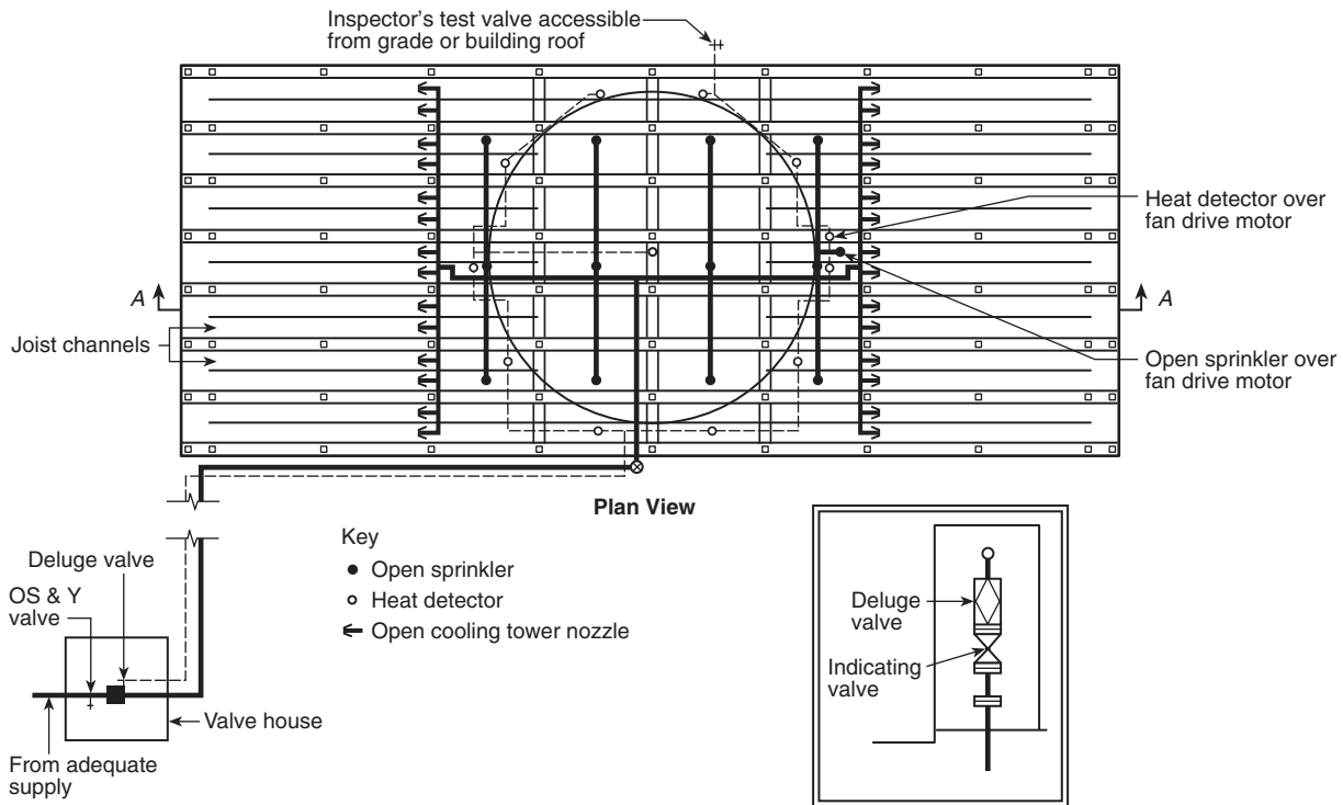
FIGURE A.21.24.2(a) Plan View, Typical Deluge Fire Protection Arrangement for Crossflow Towers. [214:Figure A.5.2.4.2(a)]
