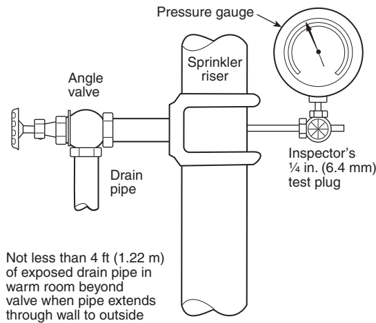
FIGURE 8.16.2.4 Drain Connection for System Riser.
