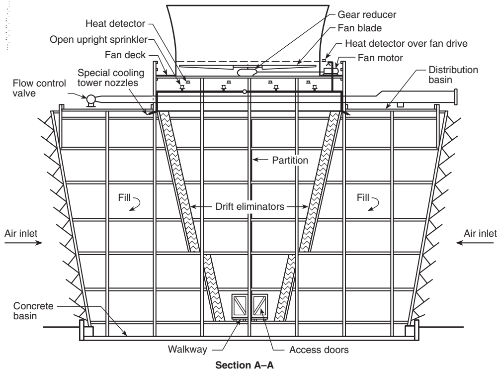
FIGURE A.21.24.2(b) Section View, Typical Deluge Fire Protection Arrangement for Crossflow Towers. [214:Figure A.5.2.4.2(b)]
