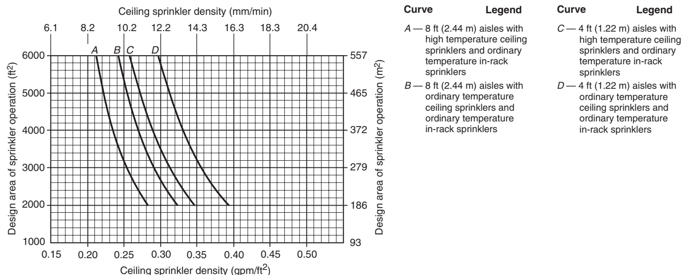
FIGURE 16.2.1.3.2(f) Single- or Double-Row Racks — 20 ft (6.1 m) High Rack Storage — Sprinkler System Design Curves — Class III Encapsulated Commodities — Conventional Pallets.
