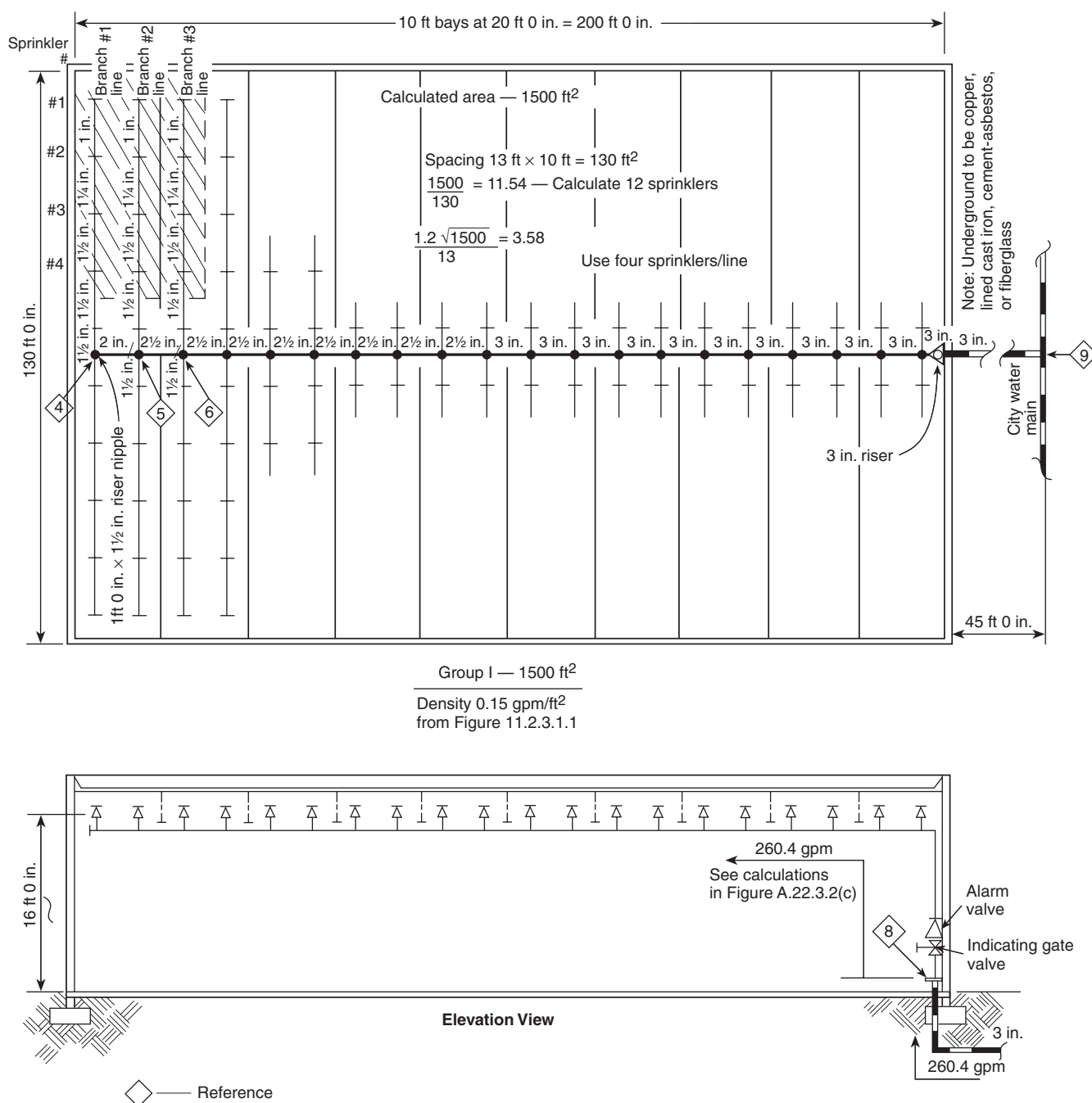
FIGURE A.22.3.2(b) Hydraulic Calculation Example (Plan View and Elevation View).
