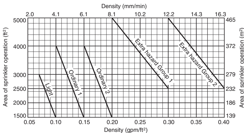
FIGURE 11.2.3.1.1 Density/Area Curves.
