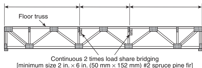
FIGURE A.3.7.2(c) Examples of Wood Truss Construction.
