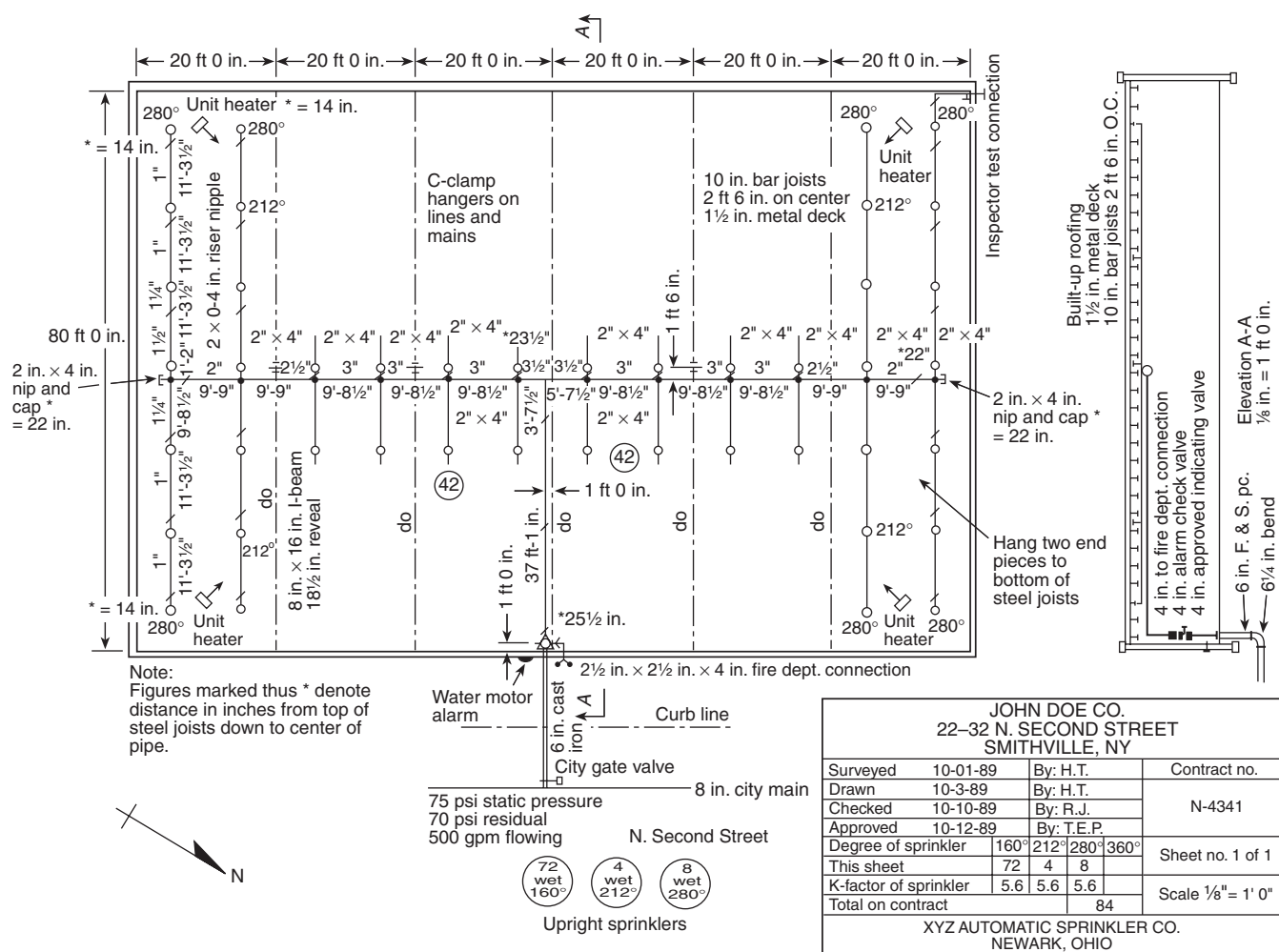
FIGURE A.22.1.1 Typical Working Plans.
