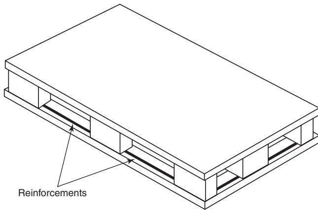
FIGURE A.3.9.1.17(b) Assembled Reinforced Plastic Pallet.
